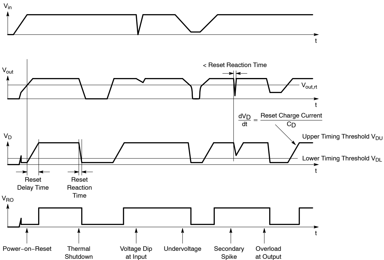
Figure 35. Reset Timing
